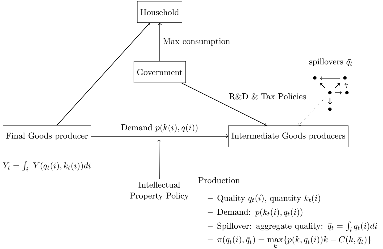
FIGURE 1: MODEL SUMMARY
