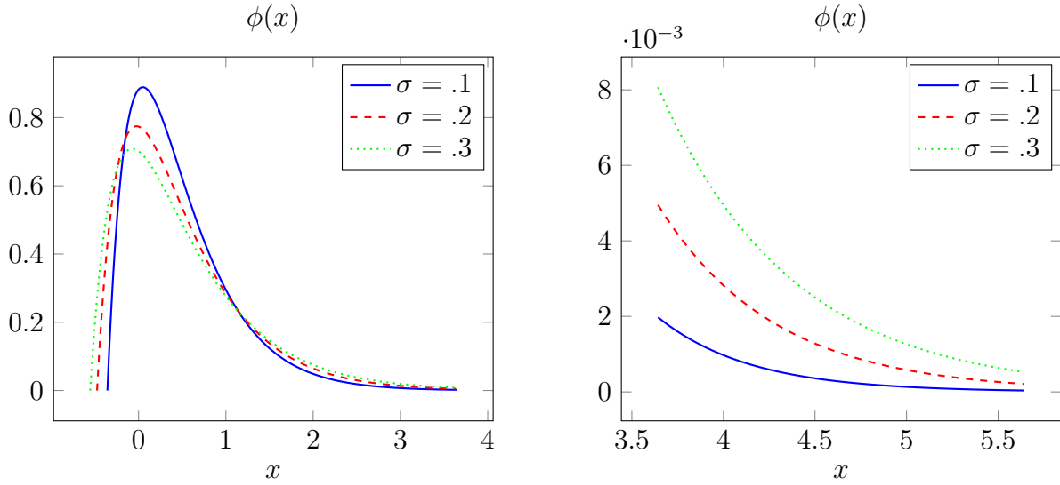
Figure 4. The stationary distribution of log-productivity for \sigma = .1, .2, and .3 . Parameter values: r = 5\%, \mu = 2\%, \lambda = .05, \rho = 3, p = 1 .
