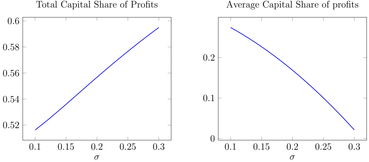
Figure 5. The total and average capital share of profit as a functions of \sigma . Parameter values: r = 5\% , \mu = 2\% , \lambda = .05 , \rho = 3 , p = 1 .
