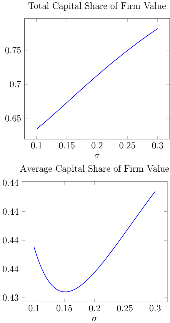
Figure 6. The total and average capital share of firm value as a functions of \sigma . Parameter values: r = 5\% , \mu = 2\% , \lambda = .05 , \rho = 3 , p = 1 .
