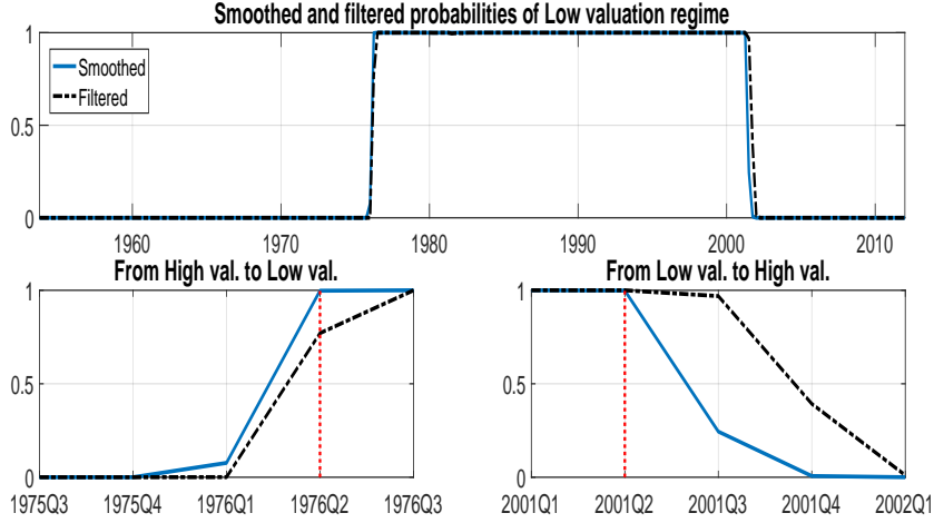
Figure A.1: Filtered and smoothed regime probabilities around switch dates.
