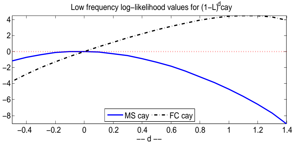
Figure A.2: Low frequency log likelihood values for (1-L)^d \text{cay}_t . The sample is quarterly and spans the period 1952:Q1 to 2013:Q3.
