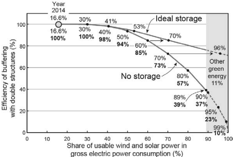
Figure 8: Efficiency losses from buffering with conventional plants and necessary storage volume for overshooting production spikes (German hourly data, 2014)
