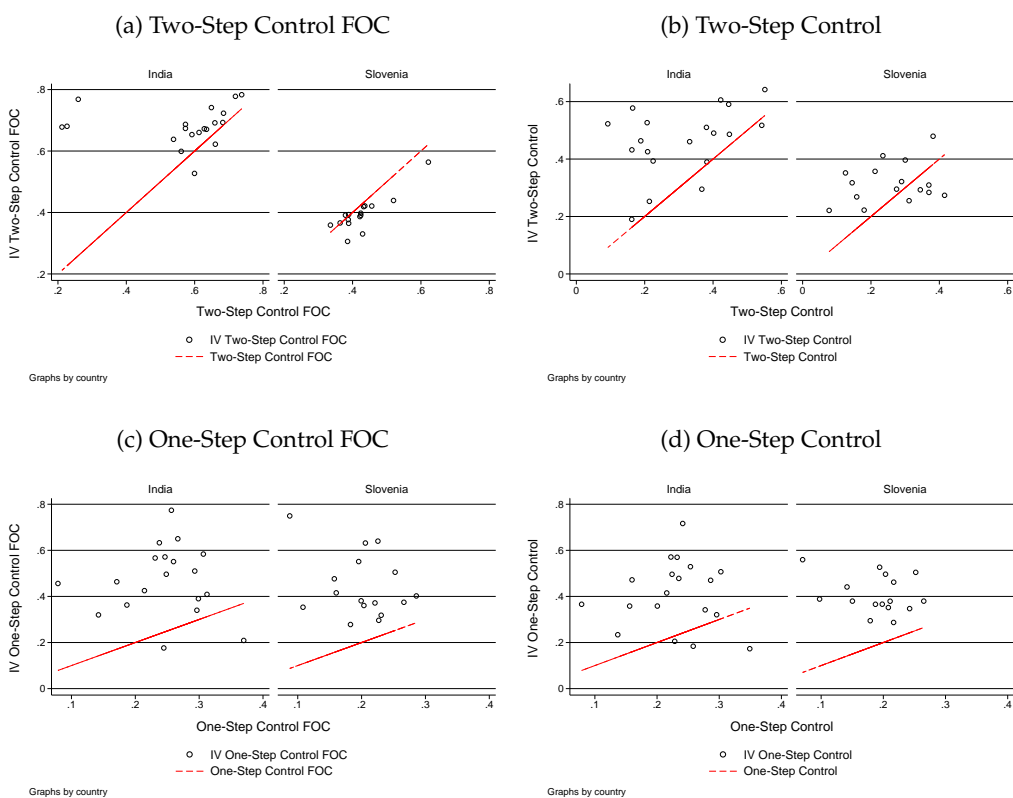
Figure 3: Industry-specific Coefficients
