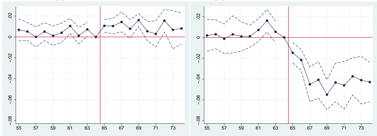
(a) 1930 coefficients
