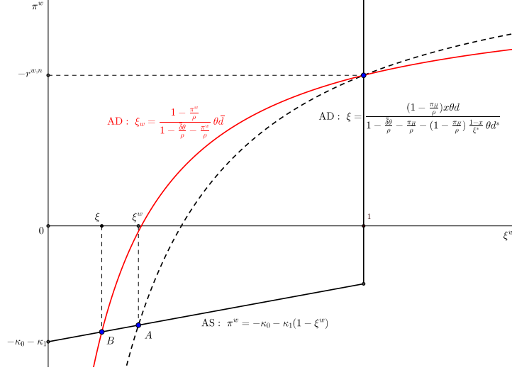
The figure reports Aggregate Supply (solid line) and Aggregate Demand (dashed line) in a symmetric equilibrium, when \kappa_0 = \kappa_0^* and \kappa_1 = \kappa_1^* . The red solid line represents the home AD curve in the asymmetric equilibrium with \xi^* = 1 .
