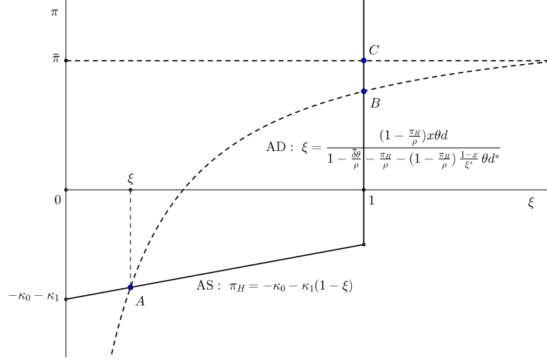
The figure reports Aggregate Supply (solid line) and Aggregate Demand (dashed line), for a given value of Foreign's output gap, \xi^* .
