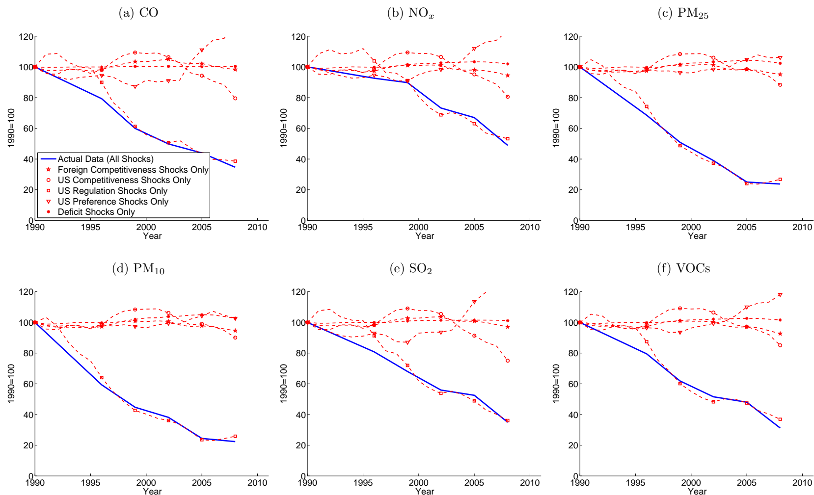
Figure 3: Counterfactual U.S. Manufacturing Pollution Emissions Under Subsets of Shocks, 1990-2008
