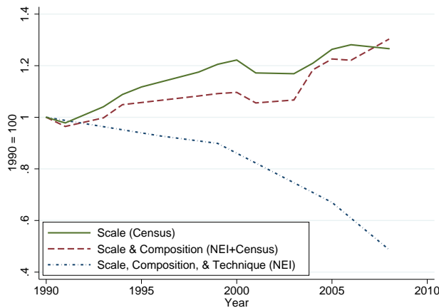
Figure 2: Nitrogen Oxides Emissions From United States Manufacturing
