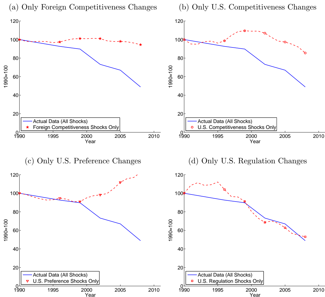
Figure A5: Counterfactual U.S. Manufacturing Emissions of \text{NO}_x Under Subsets of Shocks, 1990-2008
