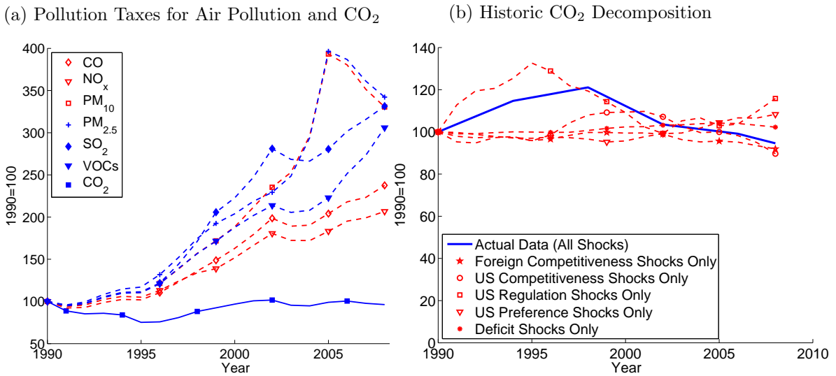
Figure 5: Analysis of Carbon Dioxide Emissions
