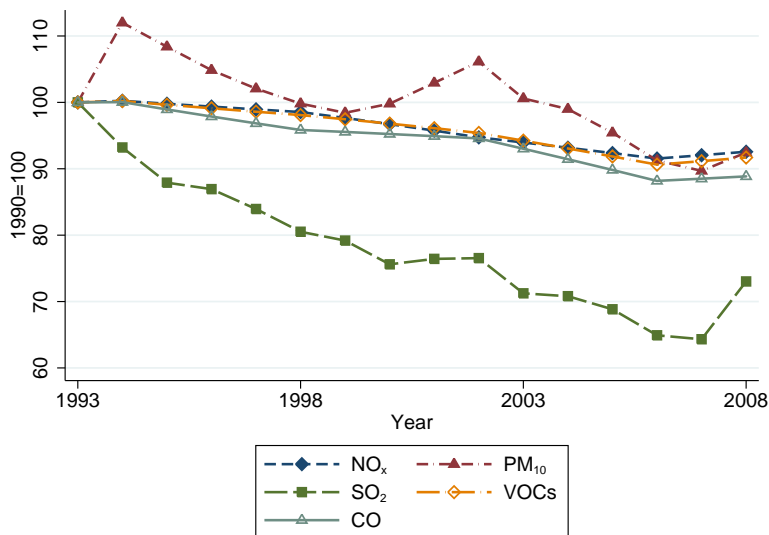
Figure A8: Potential Pollution Per BTU from Fossil Fuel Combustion, All Manufacturing, 1993-2008
