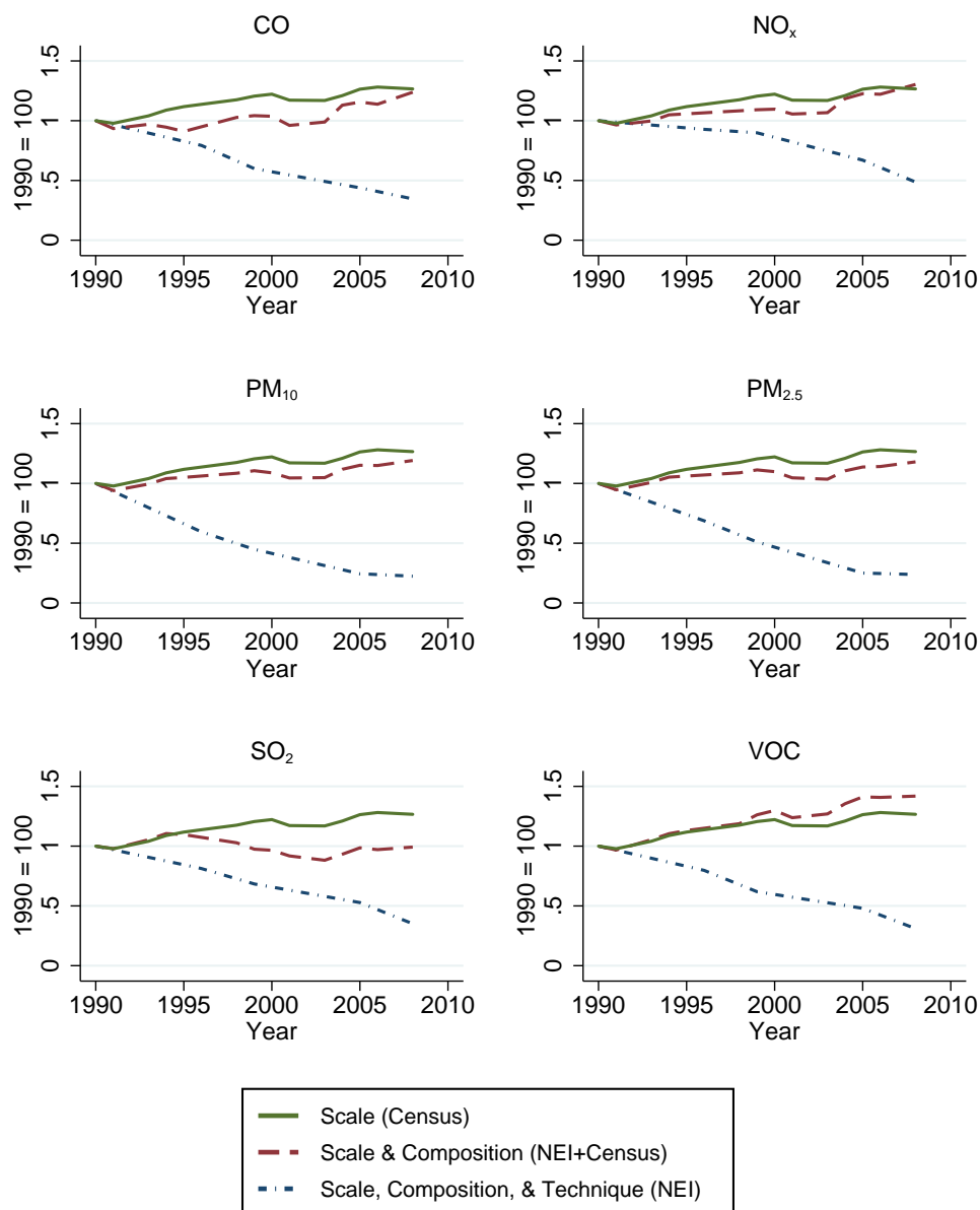
Figure A2: Emissions Statistical Decomposition From United States Manufacturing
