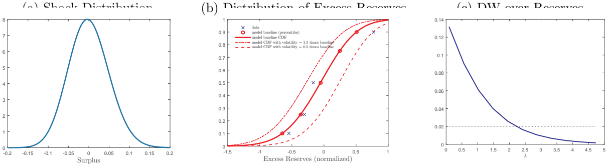
Figure 3: Shock distribution, parameters and moments
