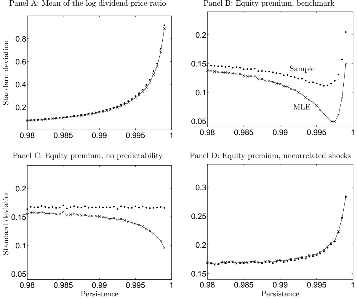
Figure 3: Standard deviation of estimators of the mean of the log-dividend price ratio (Panel A) and of the equity premium (Panels B–D). Estimators are the sample mean (dots) and maximum likelihood (crosses). For each value of the autocorrelation \theta , we simulate 10,000 monthly samples and calculate the standard deviation of estimates across samples. Parameters other than \theta are set equal to their maximum likelihood estimates with the following exceptions. In Panel B, the predictive coefficient is bias-corrected. In Panel C, the predictive coefficient is set equal to zero. In Panel D, the predictive coefficient is bias-corrected and the correlation of the shocks is set equal to zero.
