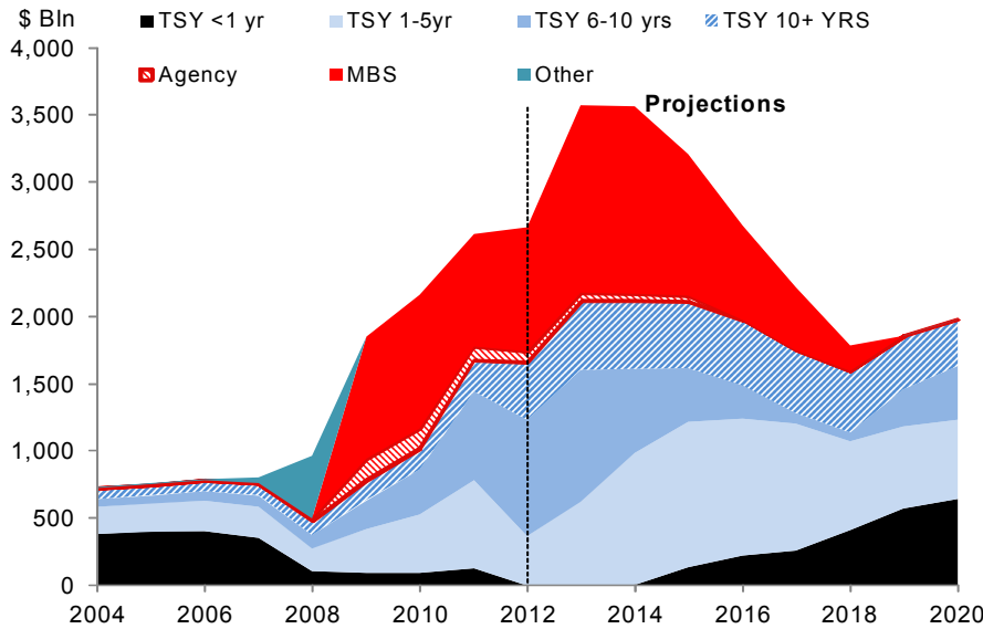
Figure 4.1. Baseline assets
