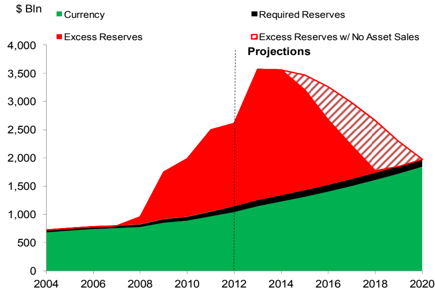
Figure 4.3 Baseline liabilities
