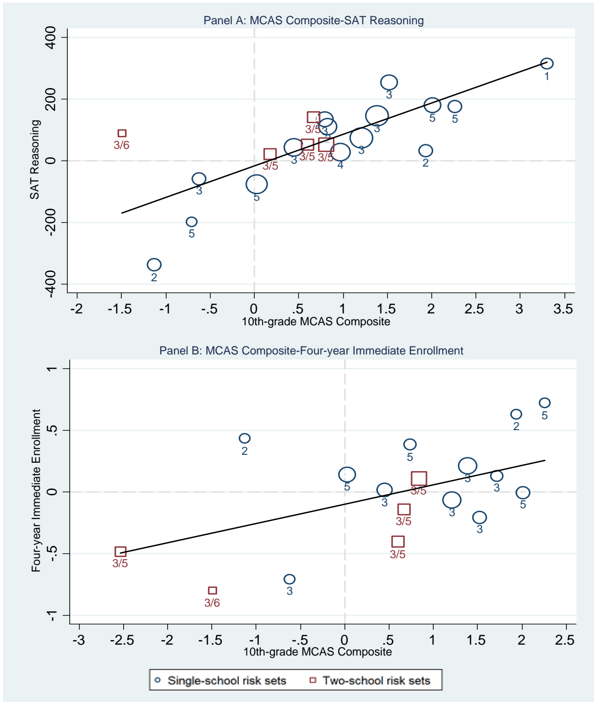
Figure 3: Lottery Estimates of Effects within Risk Sets
