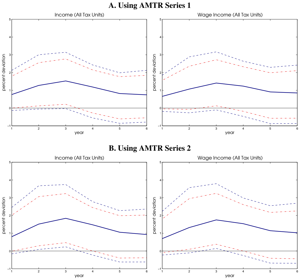
Figure D.1 Response to unit shock to the log net-of-tax rate. Broken lines are 90% and 95% confidence bands based on 10,000 wild bootstrap replications.
