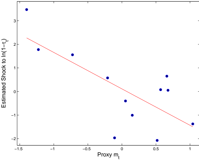
Figure 3 Proxy and Shock to \ln(1 - \tau_t)
