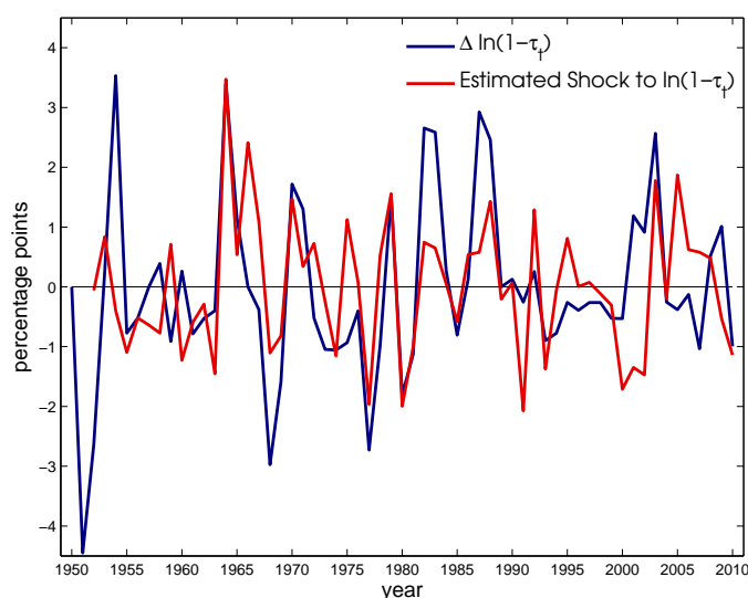
Figure 5 SVAR-identified shock and changes in the log net-of-tax rate.
