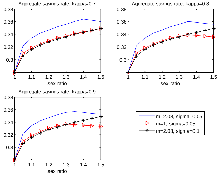
Figure 1: Economy-wide savings rate vs sex ratio
