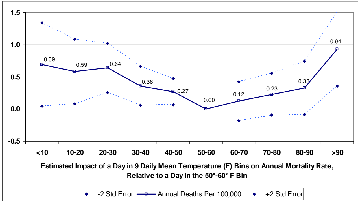
Figure 1: Estimated Relationship Between Annual Age-Adjusted Mortality Rate Per 100,000 and Average Daily Temperature in the United States, 1968-2002
