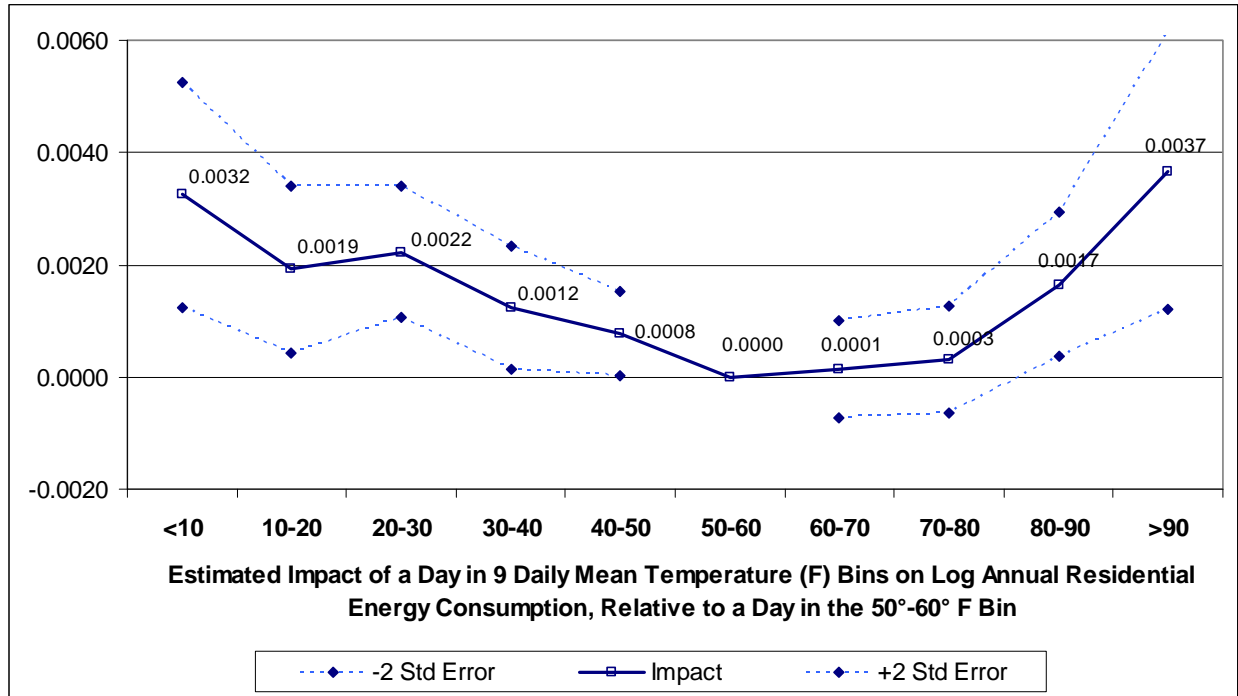
Figure 2: Estimated Relationship Between Log Residential Energy Consumption and Average Daily Temperature, 1968-2002
