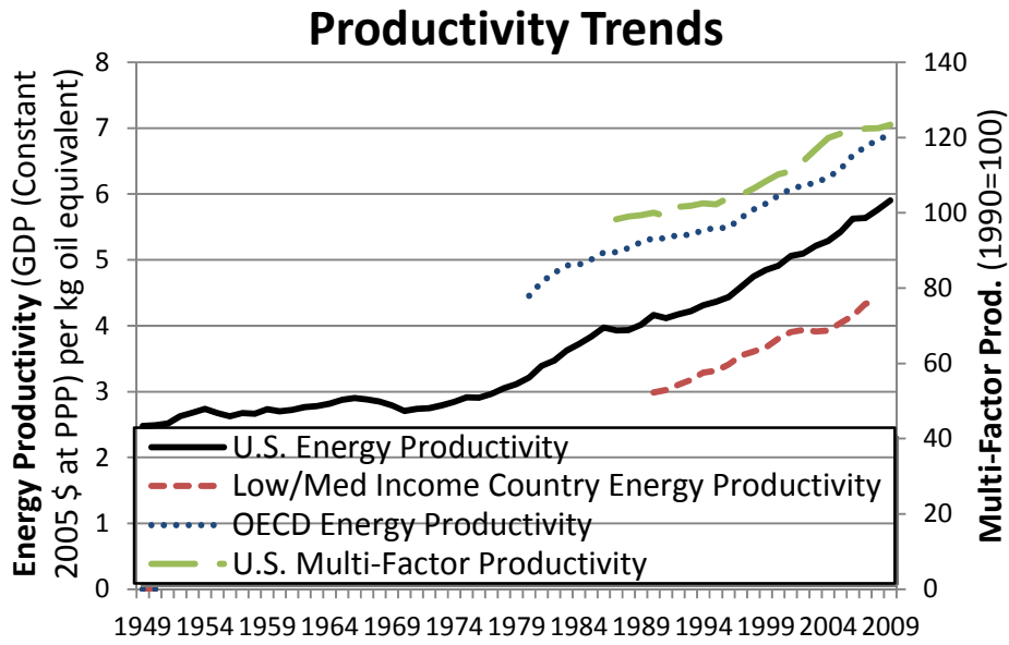
Figure 2: Productivity Trends
