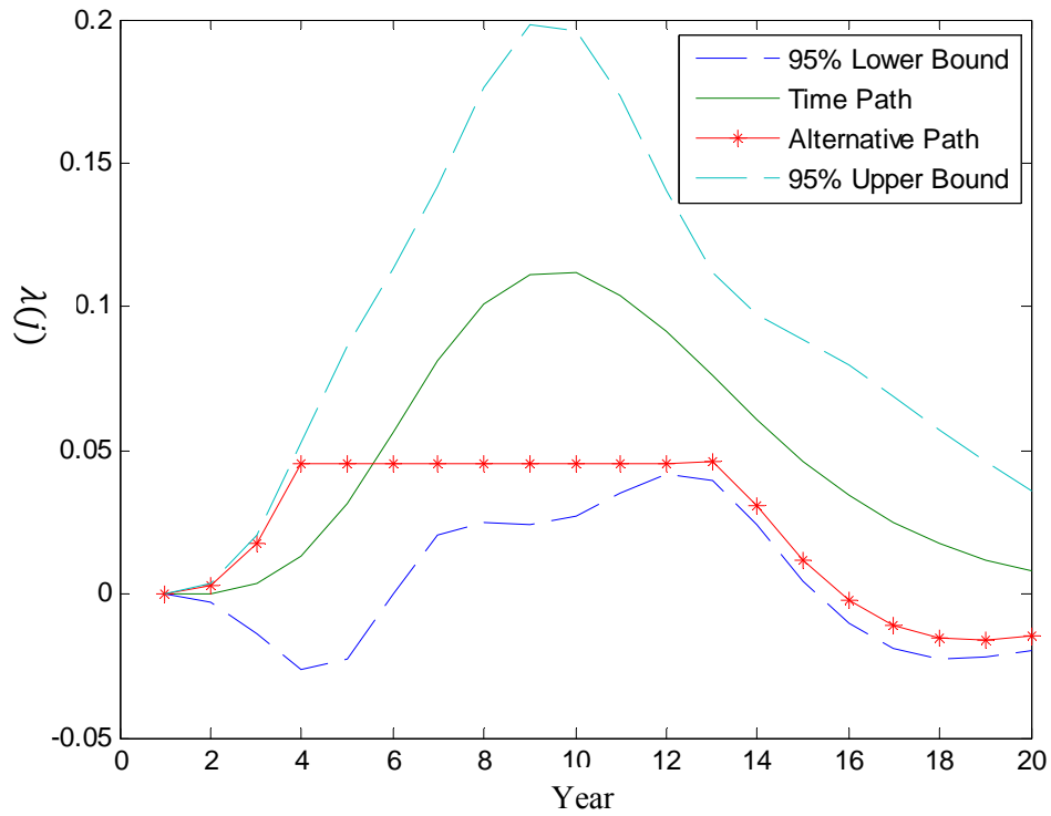
Figure 3: Long-term Effect of DSM Spending from the Baseline Model
