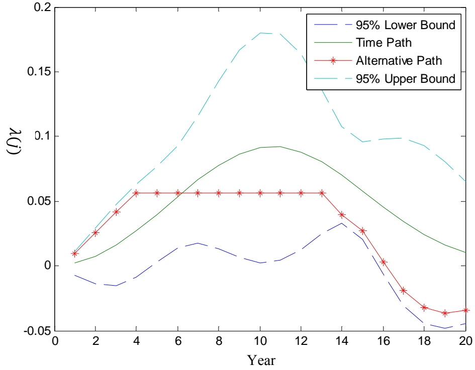
Figure 4: Long-term Effect of DSM Spending using Weibull Distribution
