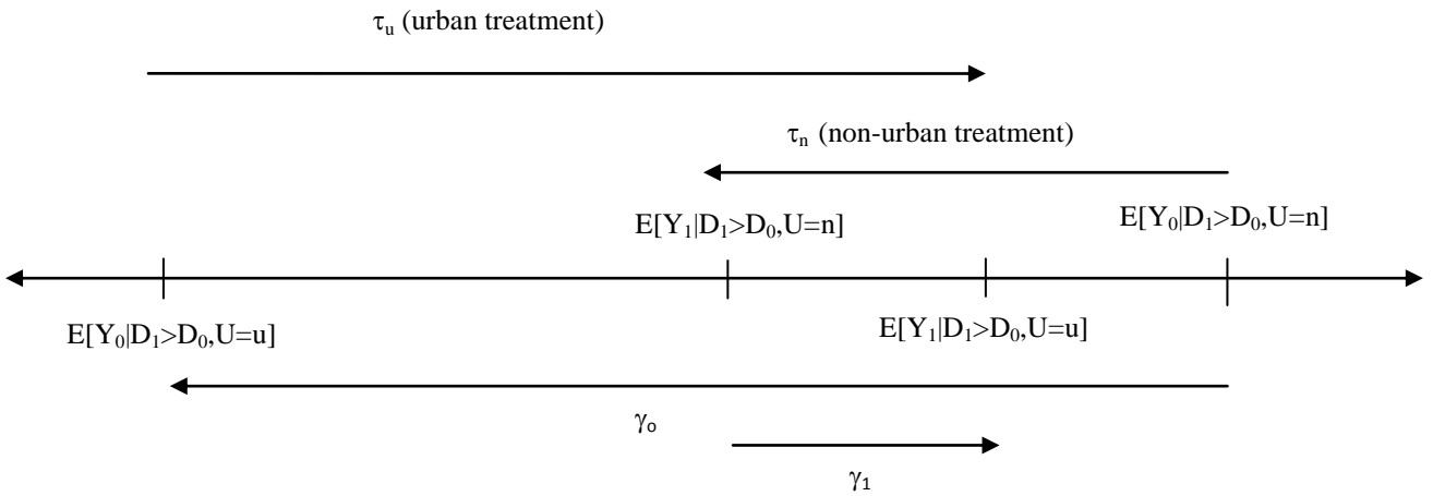
Figure 1: Urban Gaps on Treatment and No-Treatment Counterfactuals
