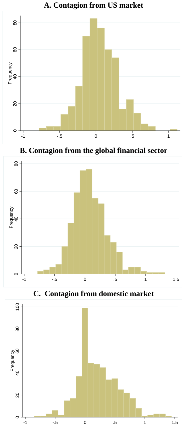
Figure 3: Distribution of Contagion Coefficients. The figures show the distribution of the contagion coefficients \gamma_{i,0} from the estimation of (11)-(12) across all 415 equity portfolios from the factor model.
