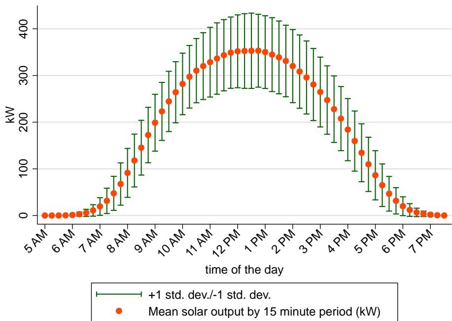
Figure C.2: Summary statistics for Tucson solar output, 2011 - 2012
