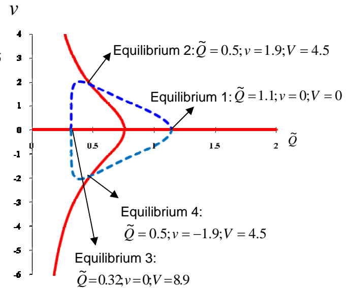
Panel B Sunspot Equilibria
