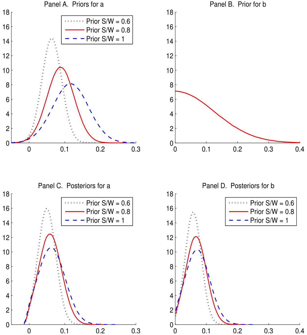
Figure 2. Prior and posterior distributions for a and b . The figure plots priors and posteriors for a and b in the function \alpha_t = a - b(S/W)_t - f , where \alpha_t is the expected active benchmark-adjusted return, (S/W)_t is the aggregate allocation to active management, and f is the fee (zero under competition). The prior for b shown in Panel B has a mean of 0.1. Three priors for a based on that value are shown in Panel A. All three have the property \text{prob}(a < 0) = 0.01 but differ with respect to the “prior S/W ”—the S/W under the fully competitive equilibrium based only on prior beliefs. Panels C and D display the posteriors obtained after updating with the mutual fund data, covering the 1962–2005 period.
