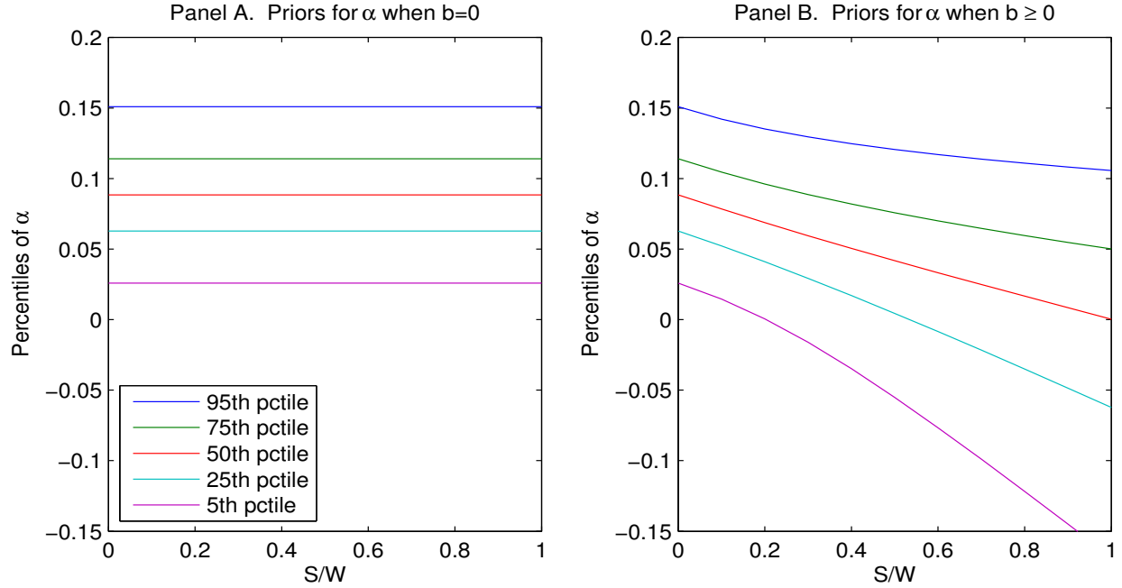
Figure 6. Priors for alpha: constant versus decreasing returns to scale. For each value of the aggregate allocation to active management ( S/W ), the figure displays percentiles of the prior distribution for alpha under constant returns to scale (Panel A) and decreasing returns to scale (Panel B), where \alpha_t = a - b(S/W)_t . The prior for a is displayed as the solid line in Panel A of Figure 2. Under constant returns to scale, the prior for b is dogmatic at b = 0 . Under decreasing returns to scale, the prior for b has a mean of 0.1 and is displayed in Panel B of Figure 2.
