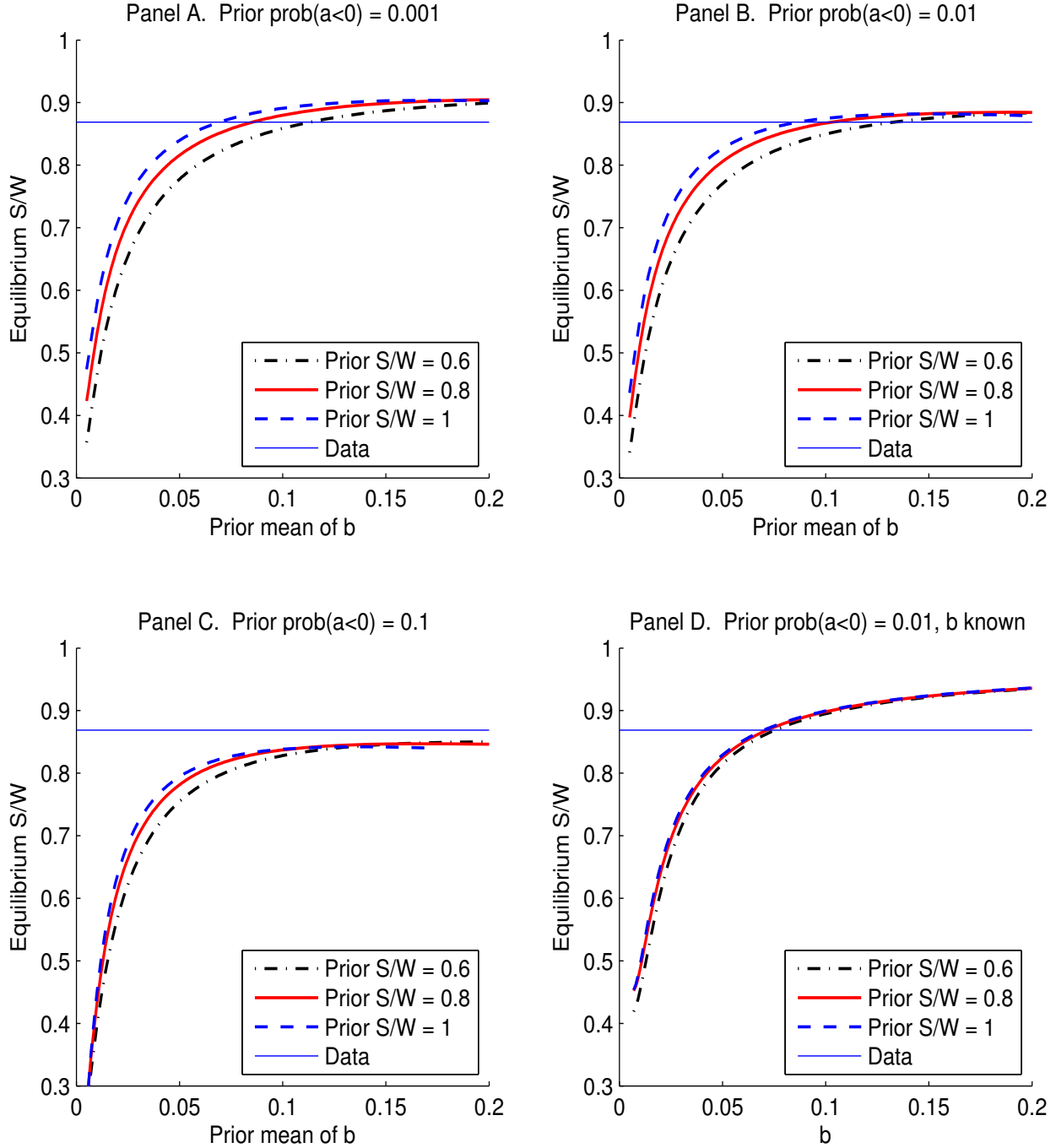
Figure 7. Equilibrium active allocation: robustness to priors. For alternative specifications of priors, the figure plots the fully competitive equilibrium aggregate allocation to active management ( S/W ), which appears as the solid curve in Figure 5 under the original prior specification. Panel B maintains the original specification \text{prob}(a < 0) = 0.01 and considers three values—0.6, 0.8, and 1.0—for the “prior S/W ,” which is the equilibrium allocation based only on prior beliefs. The same three prior S/W values are then used with each of two alternative values of \text{prob}(a < 0) : Panel A uses \text{prob}(a < 0) = 0.001 , and Panel C uses \text{prob}(a < 0) = 0.1 . Panel D treats the case in which b is known with certainty to equal the value on the horizontal axis; this case specifies \text{prob}(a < 0) = 0.01 and considers the same three prior S/W values.
