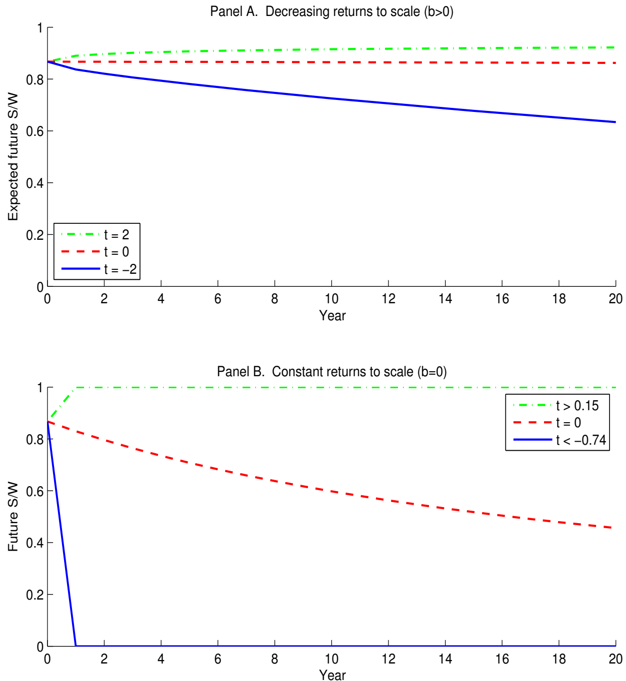
Figure 8. Expected future industry size conditional on given future performance. This figure plots the expected values of S/W , the fully competitive equilibrium aggregate allocation to active management, over 20 future years for different t -statistics of the future sample estimate of the active industry's alpha. Panel A plots the expected values of S/W conditional on future t -statistics of -2, 0, and 2 under decreasing returns to scale. In this case, future active returns are simulated based on the posteriors of a and b represented by the solid lines in Figure 2. Panel B plots the future values of S/W implied by three sets of future t -statistics, t > 0.15 , t = 0 , and t < -0.74 , under constant returns to scale. In this case, b = 0 and the distribution of a is normal with the same mean and variance as the posterior distribution of \alpha in Figure 4.
