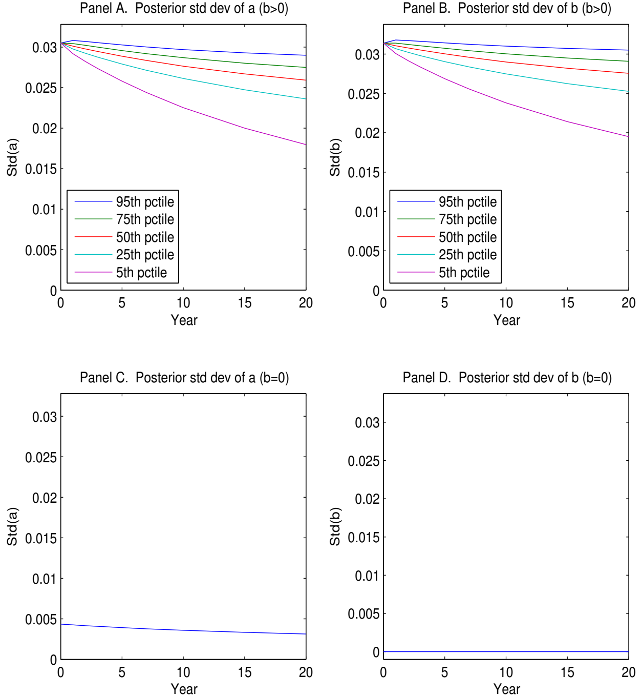
Figure 9. Speed of learning about a and b . Panels A and B plot the evolution of selected percentiles of the distributions of the posterior standard deviations of a and b , respectively, over 20 future years under decreasing returns to scale. In this case, future active returns are simulated based on the posteriors of a and b represented by the solid lines in Figure 2. Panel C plots the evolution of the posterior standard deviation of a over 20 future years under constant returns to scale. In this case, b = 0 and the distribution of a is normal with the same mean and variance as the posterior distribution of \alpha in Figure 4. Panel D simply indicates that the posterior standard deviation of b under constant returns to scale is zero.
