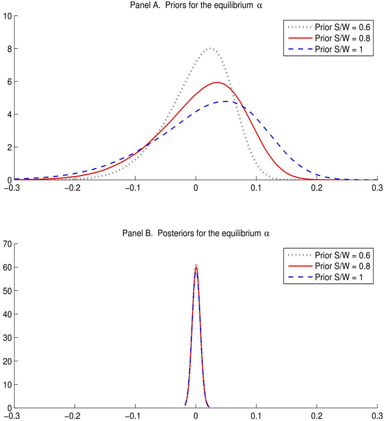
Figure 4. Prior and posterior distributions for alpha. The figure displays priors (Panel A) and posteriors (Panel B) of \alpha in the fully competitive setting, where \alpha_t = a - b(S/W)_t , and (S/W)_t is the aggregate allocation to active management. The priors and posteriors of \alpha displayed here are implied by the priors and posteriors of a and b displayed in Figure 2. The prior for b has a mean of 0.1; the three priors for a , based on that value, all have the property \text{prob}(a < 0) = 0.01 but differ with respect to the “prior S/W ”—the S/W under the fully competitive equilibrium based only on prior beliefs. The posteriors are obtained by updating the priors with the mutual fund data, covering the 1962–2005 period.
