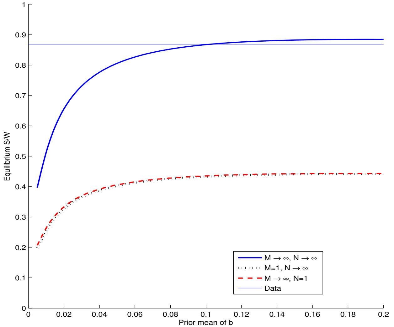
Figure 5. Equilibrium active allocation: effects of competition. For different numbers of funds ( M ) and investors ( N ), the figure plots the equilibrium aggregate allocation to active management ( S/W ) based on updated beliefs that incorporate mutual fund data for the 1962–2005 period. For each value of the prior mean of b , the prior for a is specified such that \text{prob}(a < 0) = 0.01 and the equilibrium S/W equals 0.8 in the perfectly competitive case ( M \rightarrow \infty, N \rightarrow \infty ) when based only on the prior distribution for a and b . The “Data” line represents S/W = 0.87 , the value at the end of 2005 for the mutual fund industry.
