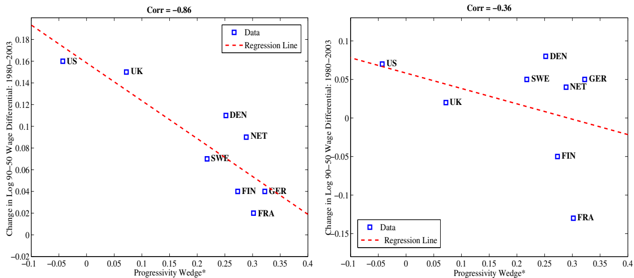
Figure 4: Progressivity Wedge* and Change in Log 90-50 (Left) and 50-10 (Right) Differentials: 1980 to 2003 . The wedge measure for country i is PW_i^*(0.5, 2.5) as defined in equation (7). Progressivity increases along the horizontal axis.
