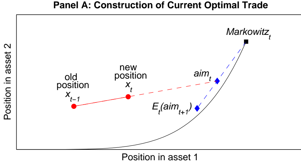
Figure 1: Optimal Trading Strategy: Aim in Front of the Target. This figure shows how the optimal trade moves the portfolio from the existing position x_{t-1} towards the aim portfolio, trading only part of the way to the aim portfolio to limit transactions costs. The aim portfolio is an average of the current Markowitz portfolio (the optimal portfolio in the absence of transaction costs) and the expected future aim portfolio, which reflects how the Markowitz portfolio is expected to mean-revert to its long-term level (the lower, left corner of the figure).
