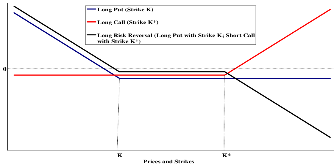
Figure 1: Option Payoffs
