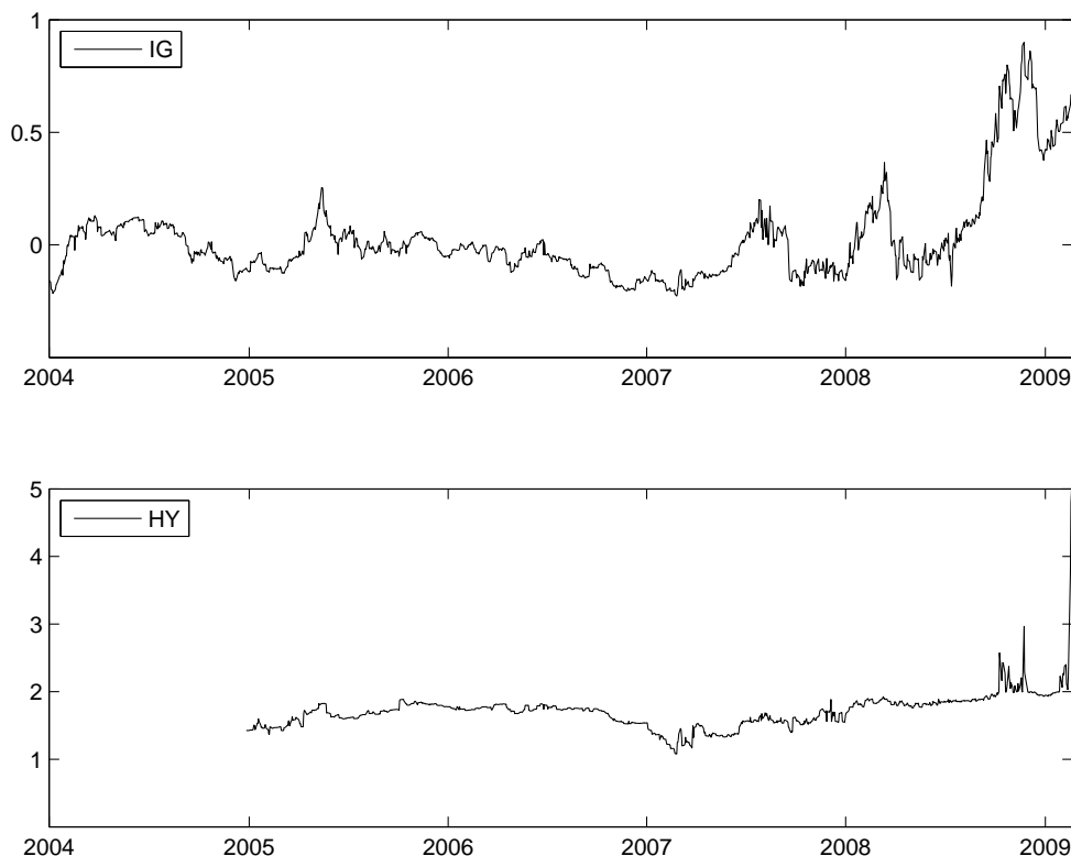
Figure 3. Implied Loss Rates for CDO Equity. The upper panel plots the implied loss rate obtained by setting the discount rate for the IG 10 equity tranche equal to the discount rate for the index bank stocks and solving for the implied discount rate. The lower panel plots the corresponding implied loss rate for the HY 10 equity tranche.
