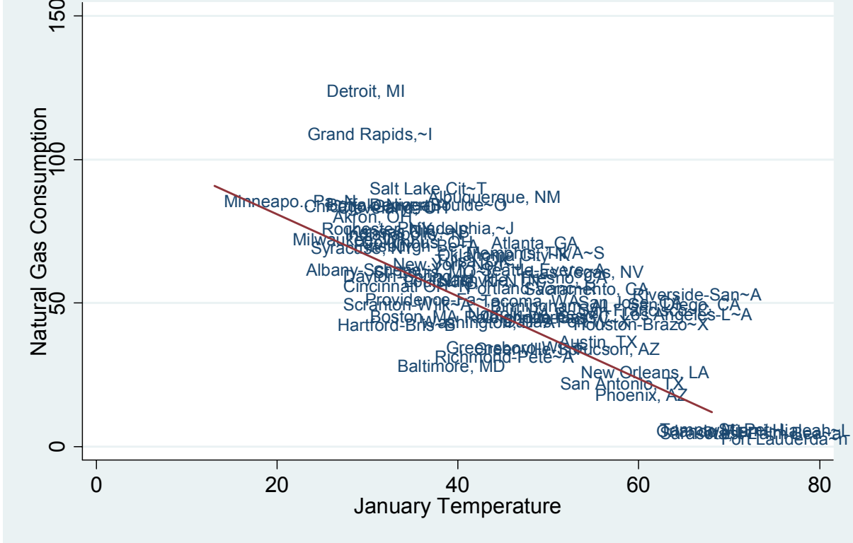
Figure 2: Relationship Between Natural Gas Consumption and January Temperature
