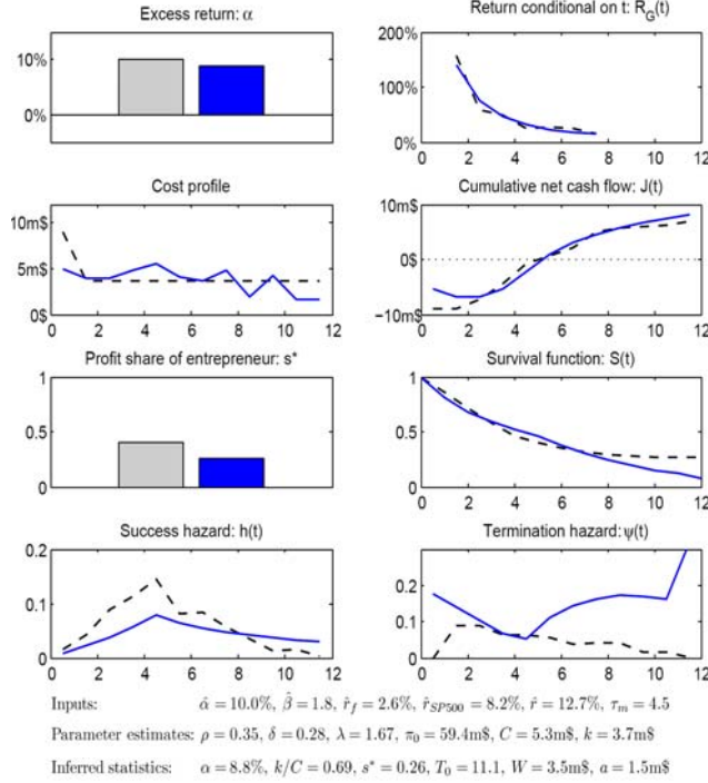
Figure 9: FIT OF THE PARETO MODEL WHEN \alpha = 0.10
