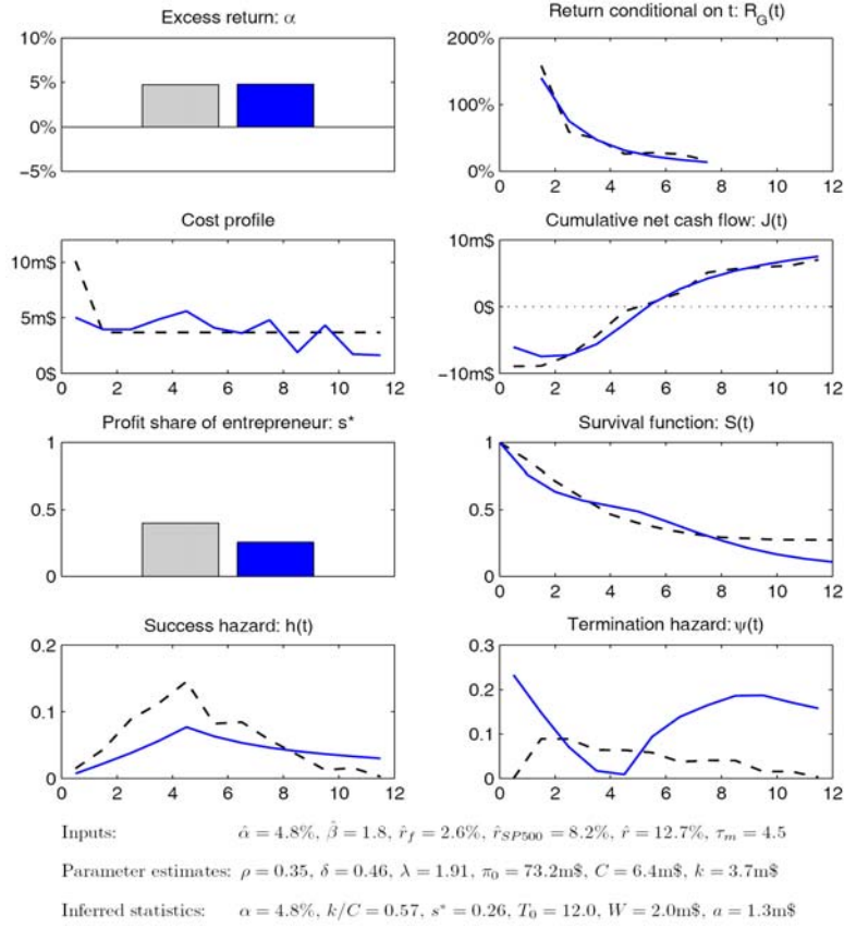
Figure 8: FIT OF THE PARETO MODEL WHEN \alpha = 0.05
