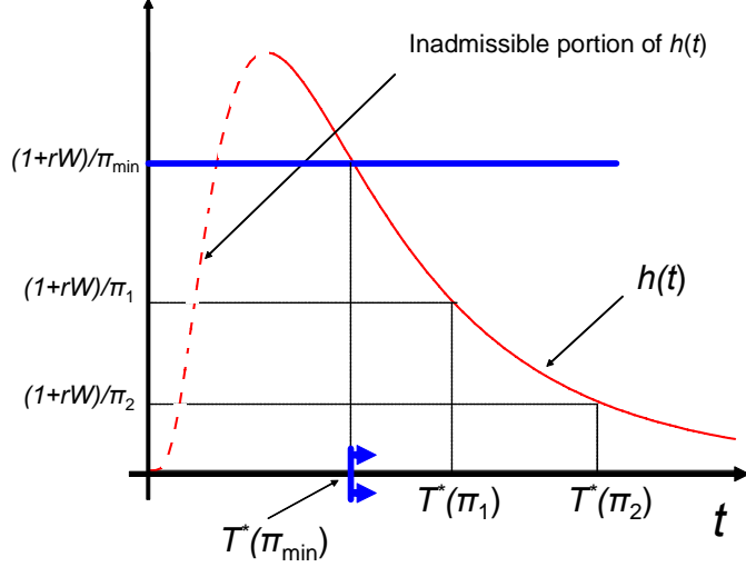
Figure 1: THE DETERMINATION OF T^*(\pi)
