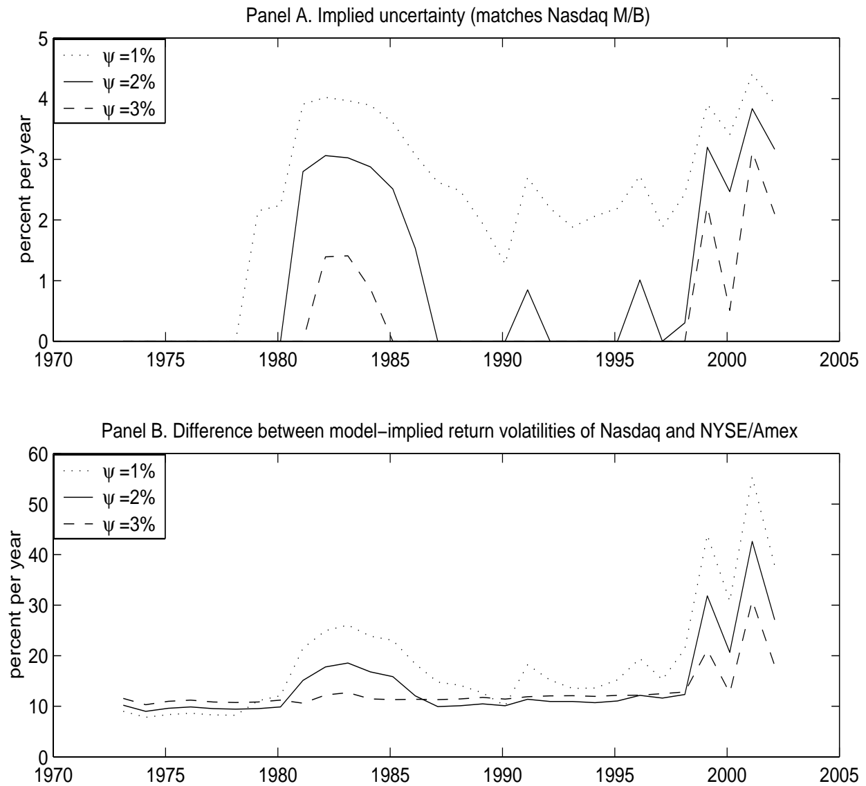
Figure 7. Implied uncertainty. Panel A plots the time series of the implied uncertainty that sets the actual M/B ratio of the Nasdaq index at the end of the current year equal to its model-implied value. Implied uncertainty is plotted for three different values of expected excess profitability. Panel B plots the model-implied difference between the return volatilities of the new and old economies.
