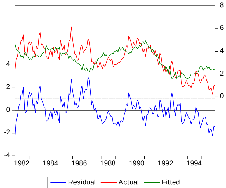
Figure 5-1: Actual value, Fitted value, and residual: call – \pi_{t-1}
