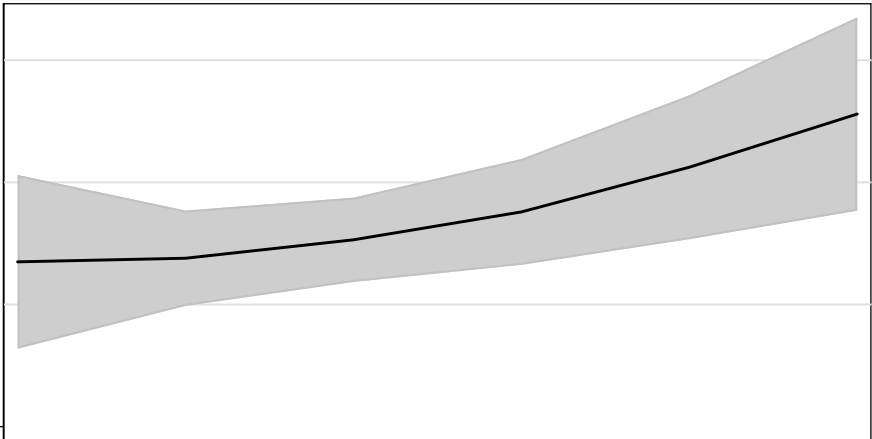
Figure 1: Integral Multipliers by Horizon, Nakamura-Steinsson Data, IV-local projection
