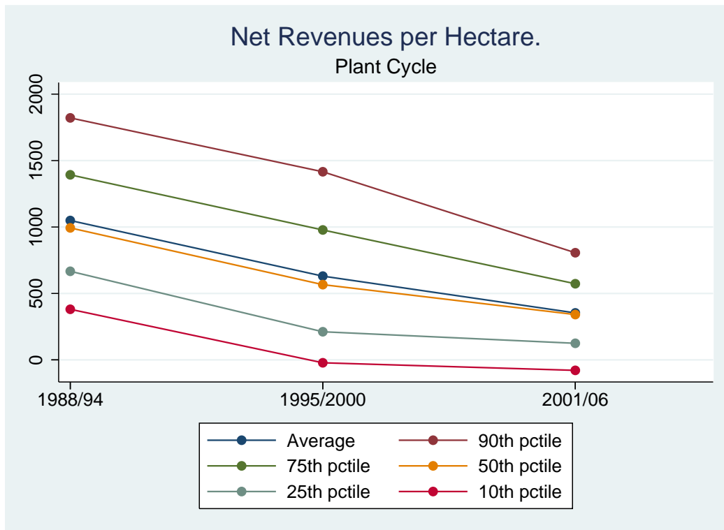
Figure 8: Net Revenues per Hectare
