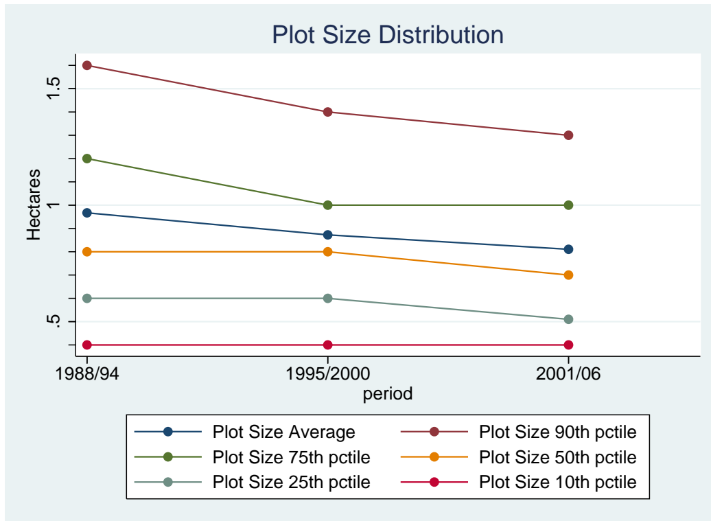
Figure 5: Plot Size Distribution
