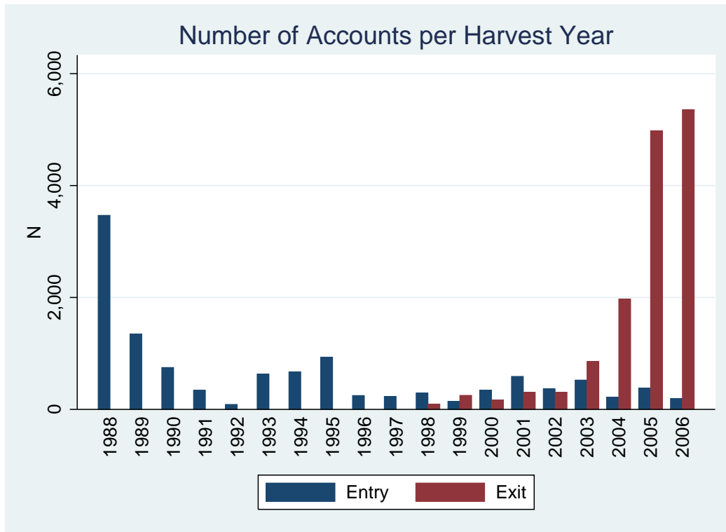
Figure 2: Entry and Exit by Harvest Year
