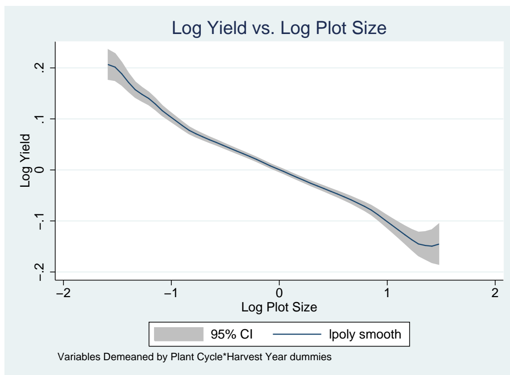
Figure 10: Log Yields vs. Plot Size
