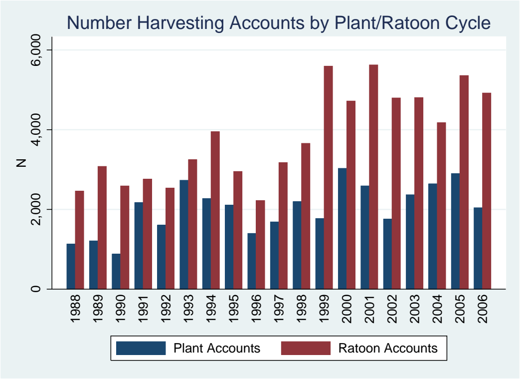
Figure 1: Number of Observations per Harvest Year by Plant Cycle
