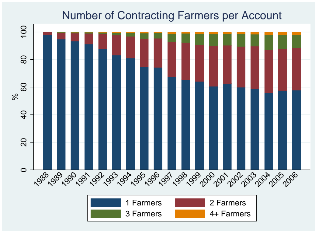
Figure 4: Number of contracting farmers per account
