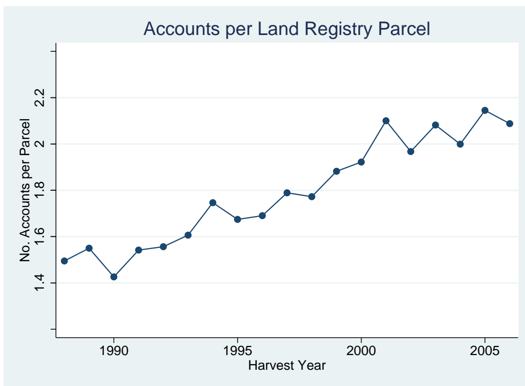
Figure 3: Number of accounts per land registry parcel
