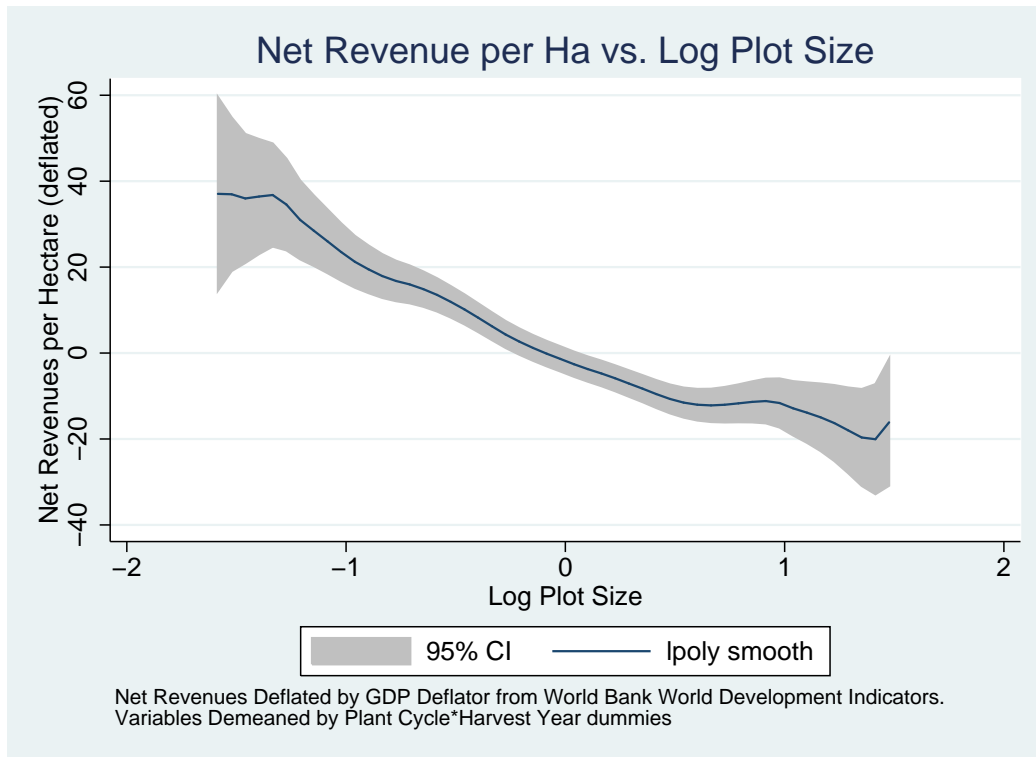
Figure 11: Net Revenues per Hectare vs. Plot Size
