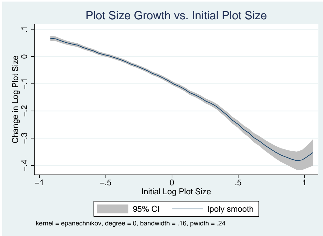
Figure 6: Size Last Harvest/Size First Harvest vs. Size First Harvest
