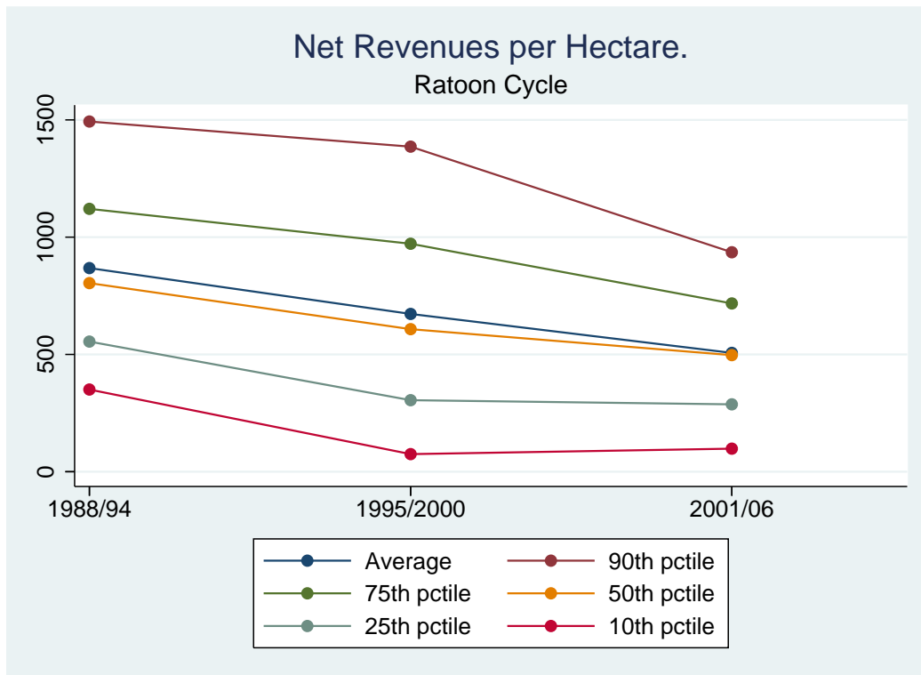
Figure 9: Net Revenues per Hectare
