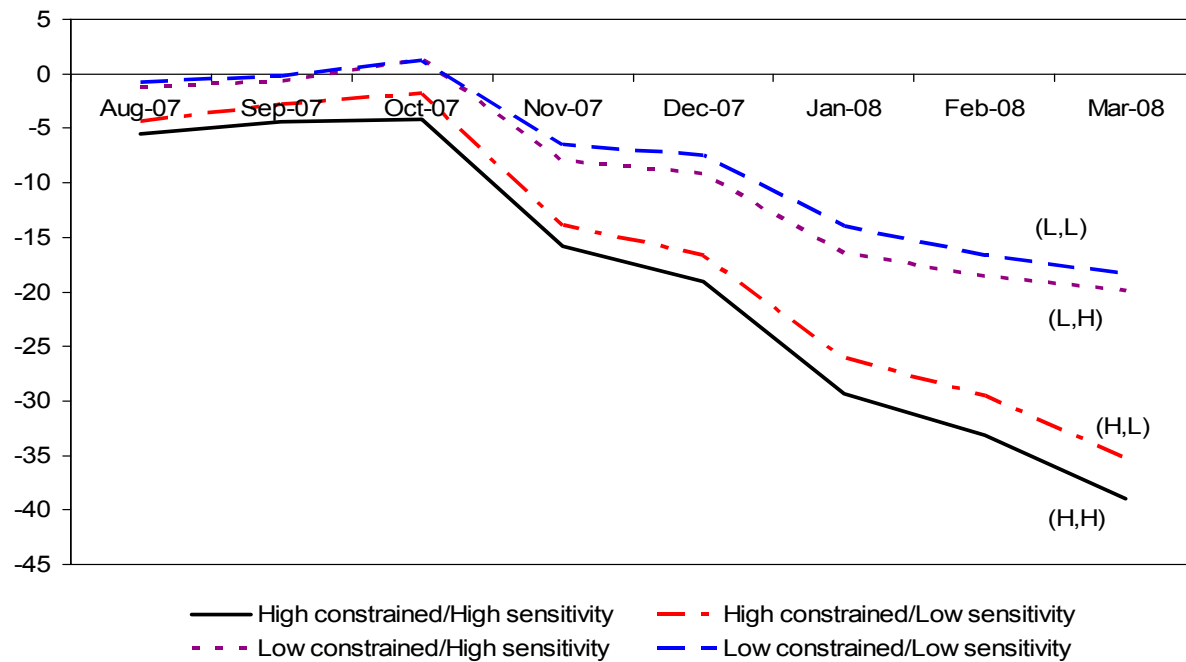
Figure 7: Key Regression Coefficients from Successively Expanding Samples
