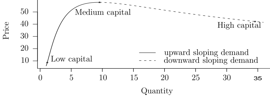
Figure 7: Simulation of Price Paths
