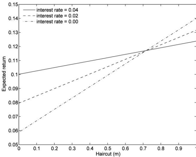
Fig. 4. Interest rate cut: the steepening of the haircut-return relationship
