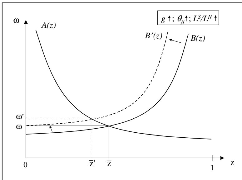
Figure 3: General Equilibrium
