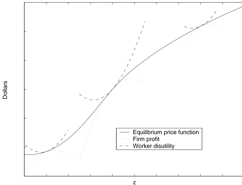
Figure 1: Optimal job choice for three worker-firm pairs
