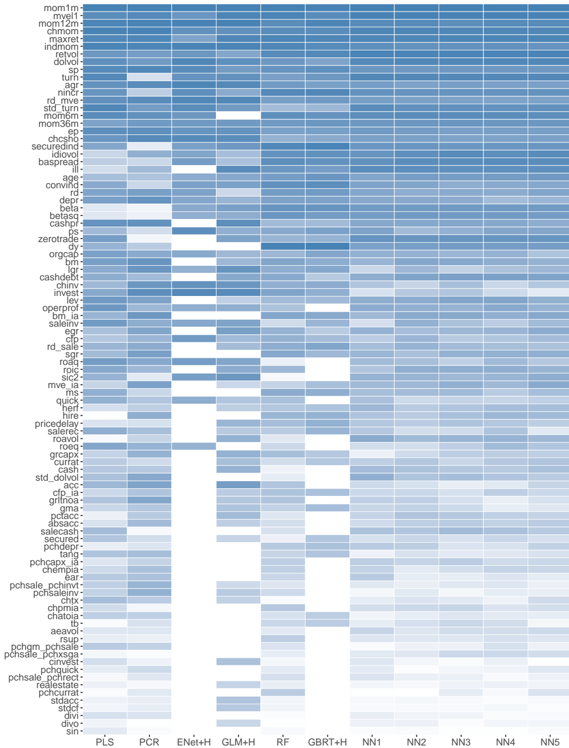
Figure 5: Characteristic Importance
