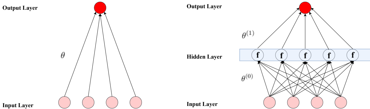
Figure 2: Neural Networks
