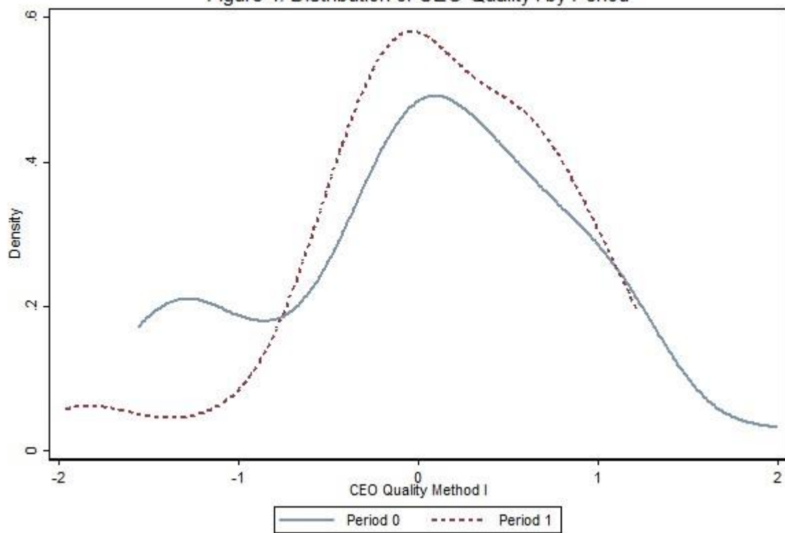
Figure 4: Distribution of CEO Quality I by Period
