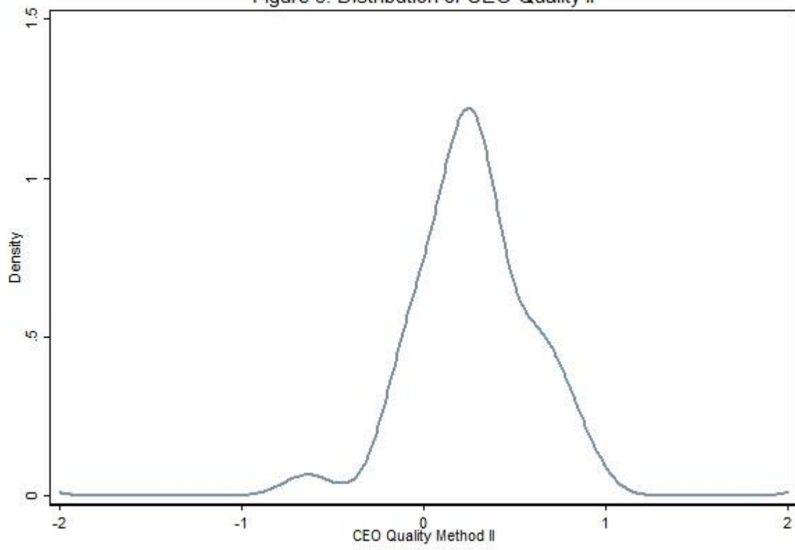
Figure 6: Distribution of CEO Quality II
