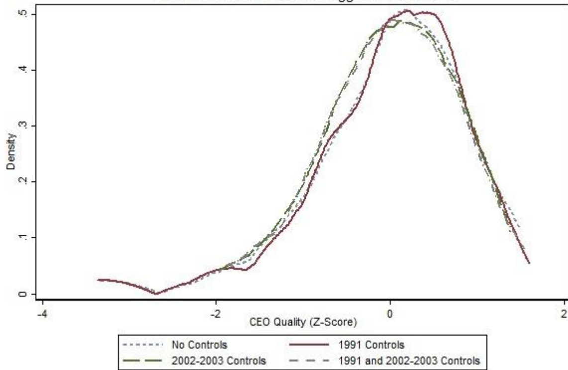
Figure 5: Distribution of CEO Quality I with Different Controls for Lagged Test Scores
