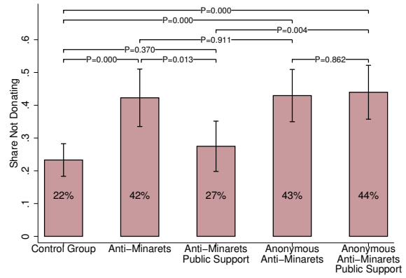
Figure 3: Auxiliary Experiments: Donation Rates Panel A
