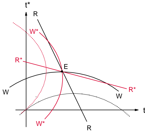
Figure 1: Nash Equilibrium of a Tariff-Setting Game
