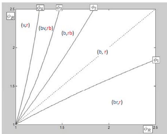
Figure 1: Equilibrium strategies under Veto for n = 5 . The colored letters in parentheses refer to the strategy of the common-value agents. The first element of each couple (in blue) refers to the strategy of z_B -agents. The second element of each couple (in red) refers to the strategy of z_R -agents. Pure strategies are denoted by single letters, mixed strategies are denoted by two letters.
