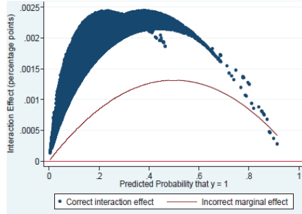
Panel A: Interaction Coefficients (LOW)
