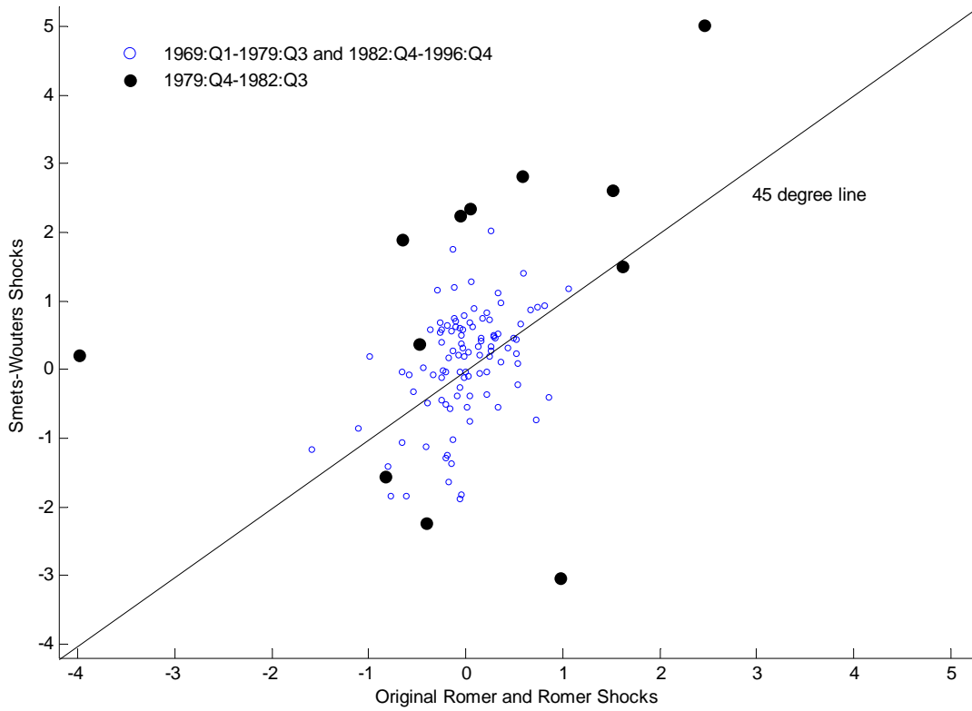
Appendix Figure 7: Original Romer and Romer Shocks vs Smets-Wouters Shocks
