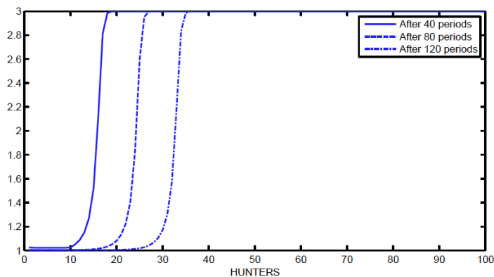
Figure 10: Evolution of hunters
