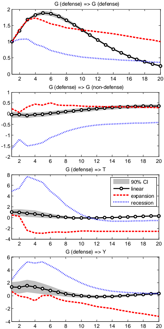
confidence bands for the linear model
