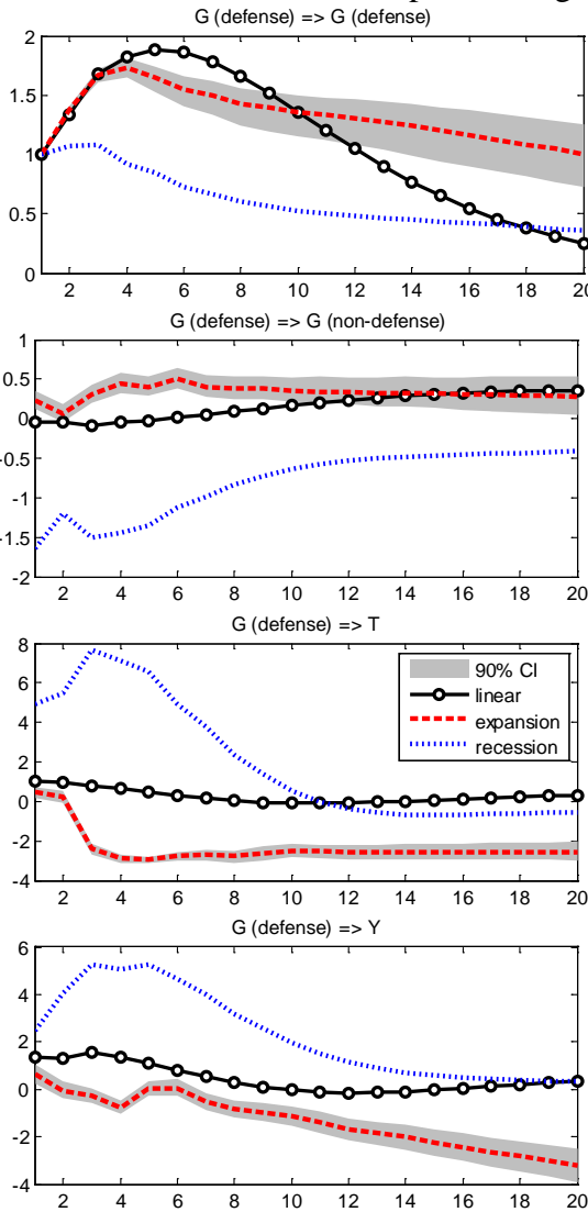
confidence bands for the expansion regime
