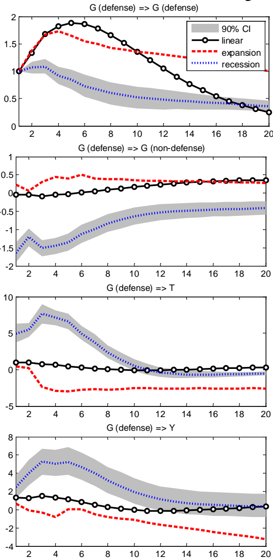
confidence bands for the recession regime
