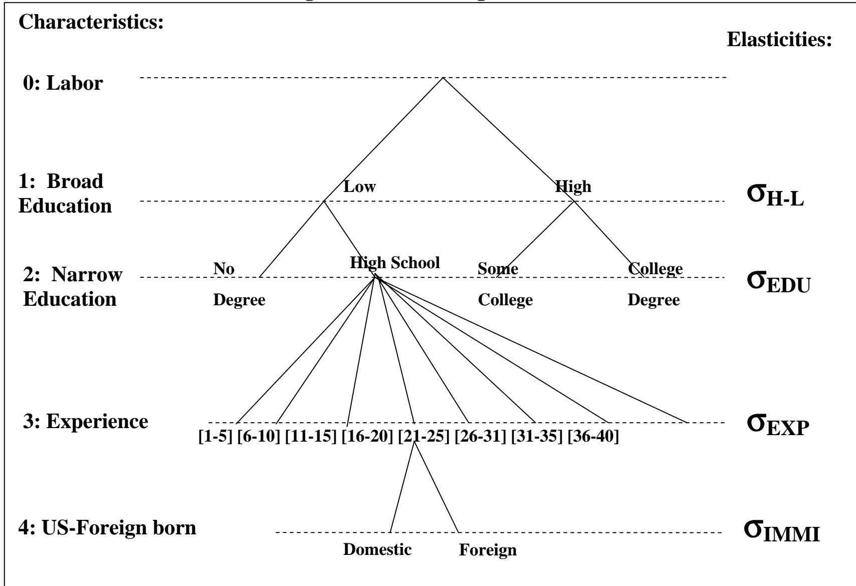
Figure 1: CES nesting structure
