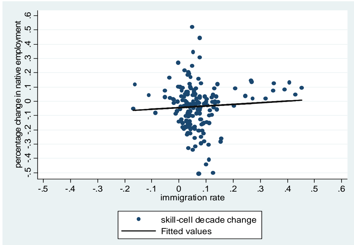
Figure 4 Native employment change and immigrant inflow California, relative to rest of US, 32 skill groups, decade changes 1960-2000 plus 2000-2005 change
