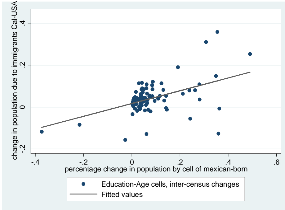
Figure A5 Mexican population change relative to the US and relative immigration to California Education-Experience cell, decade-change 1960-2005
