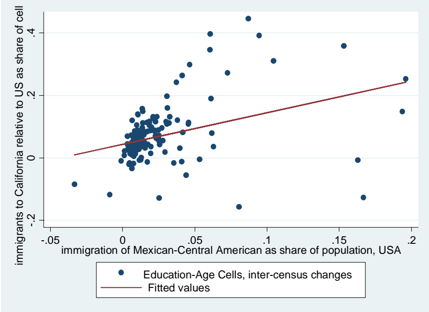
Figure A3 Mexican-Central American Immigration in the US and relative immigration to California Immigrants as percentage of the Education-Experience cell, decade-change 1960-2005
