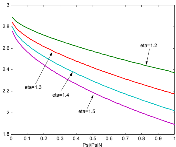
Figure 4: \rho(\psi/\psi_N|\eta)
