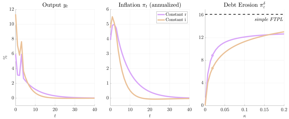
Figure B.2: Output and inflation impulse responses (left and middle) to the post-covid fiscal deficit shock (see text) and \pi_\epsilon^\delta (right) as a function of \kappa , with perfect foresight and under two different assumptions on the monetary policy reaction: fixed real rates (purple) and fixed nominal rates (orange).
